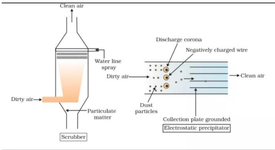
Electrostatic Precipitator
